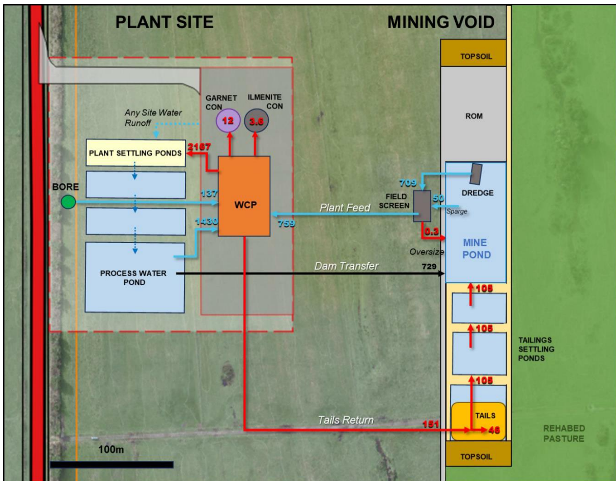
Figure 2. Site water balance diagram with flows in m 3 /hour (from Kōmanawa 2023a)
